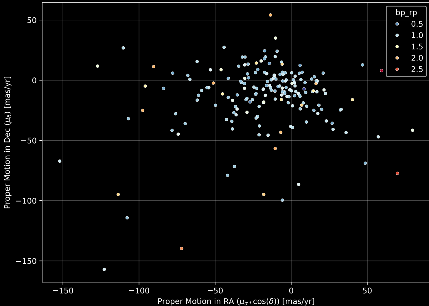
APOGEE DR17 Field: [129+66_MGA] Proper Motion Diagram (n= 187)
