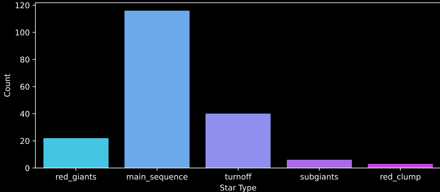
APOGEE DR17 Field: [129+66_MGA] Count plot of Star Type
