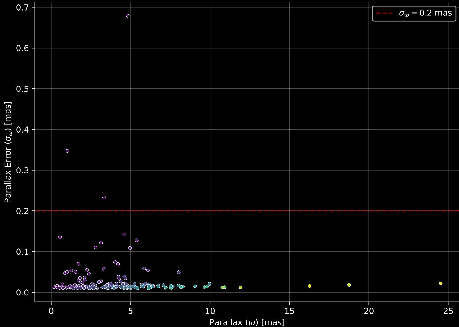
APOGEE DR17 Field: [129+66_MGA] Parallax Quality (n= 187)
