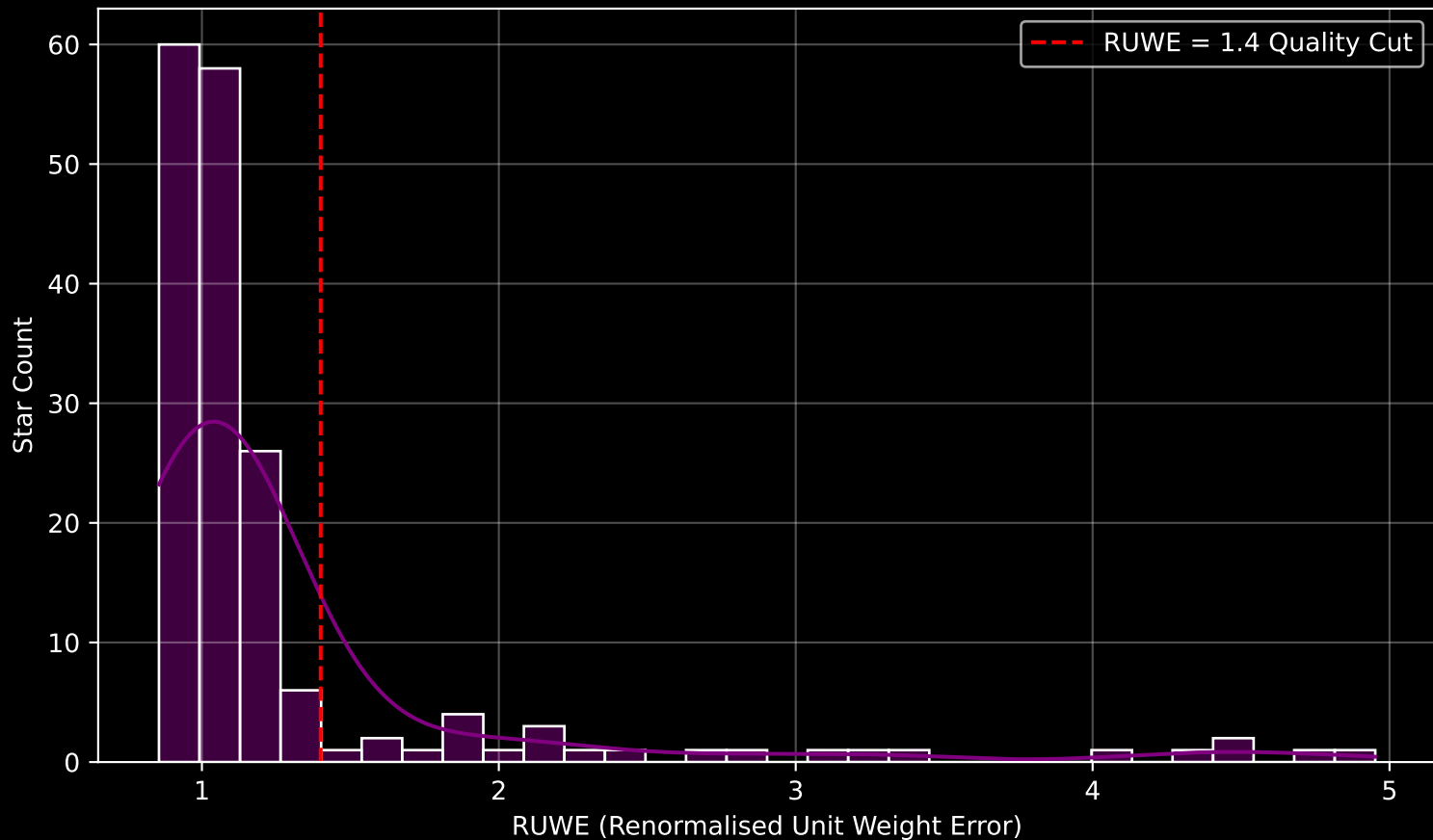
GAPOGEE DR17 Field [129+66_MGA] RUWE Distribution (n= 175)
