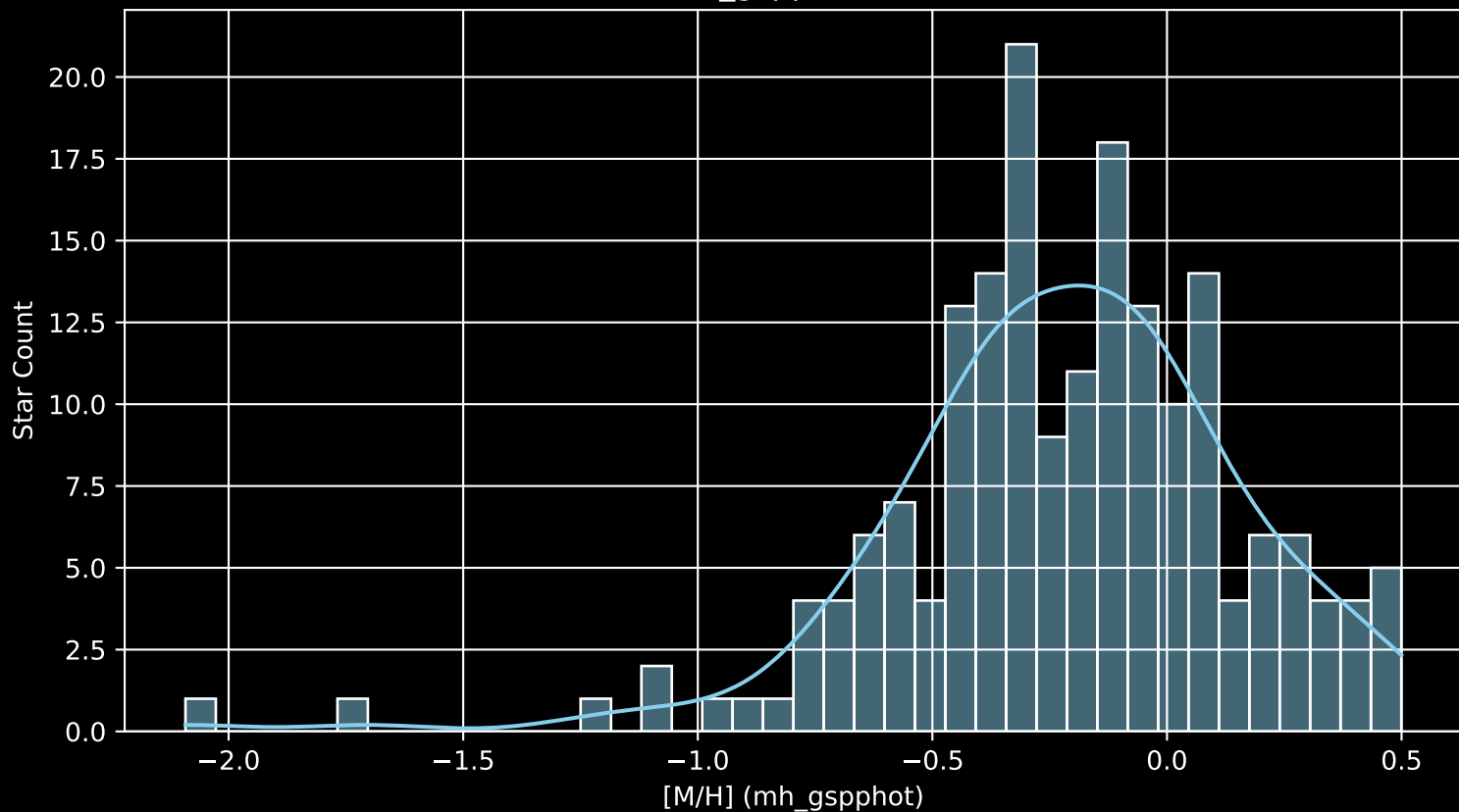
APOGEE DR17 Field: [129+66_MGA [M/H] (mh_gspphot) (n= 185)
