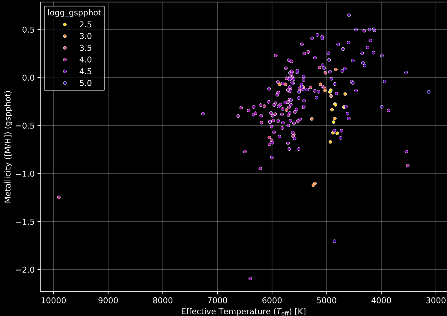
APOGEE DR17 Field: [129+66_MGA] Stellar Population Parameters (n= 187)
